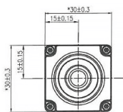
AC-AR0233-H60/ AC-AR0233-H60-60FPS
